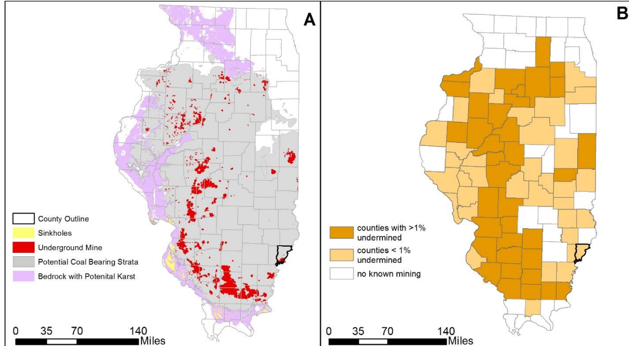
Figure 4-24. Distribution of Bedrock with Potential Coal Bearing Strata, Karst, Sinkholes and Mining Efforts
