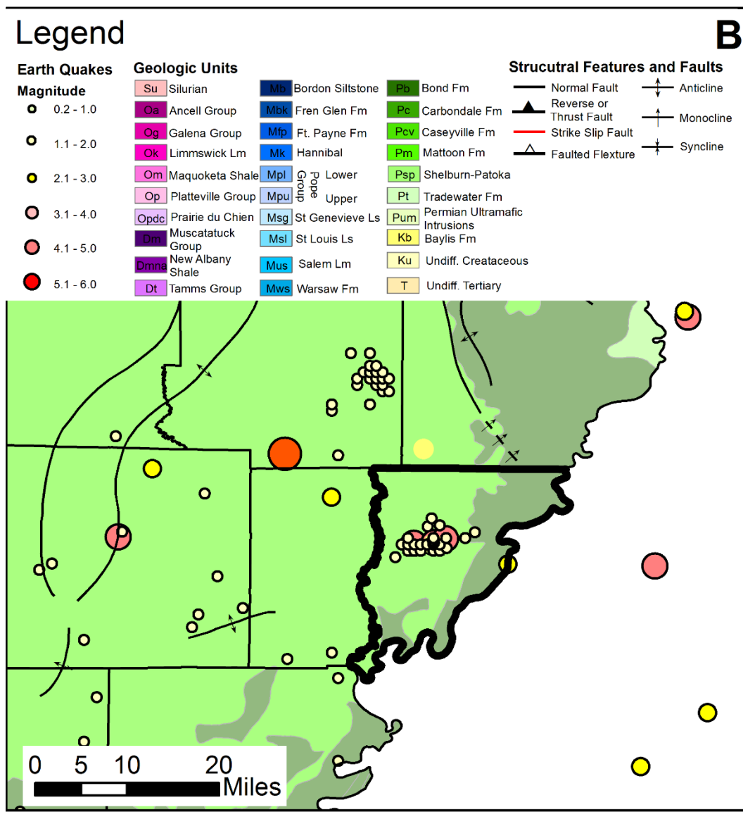
Figure 4-8. Notable Earthquakes in Illinois with Geologic and Earthquake Epicenters in Wabash County
