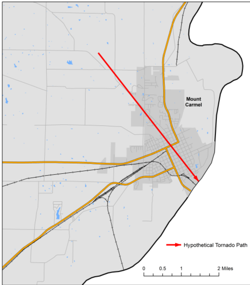
Figure 4-4. Modeled Tornado Track for Wabash County
