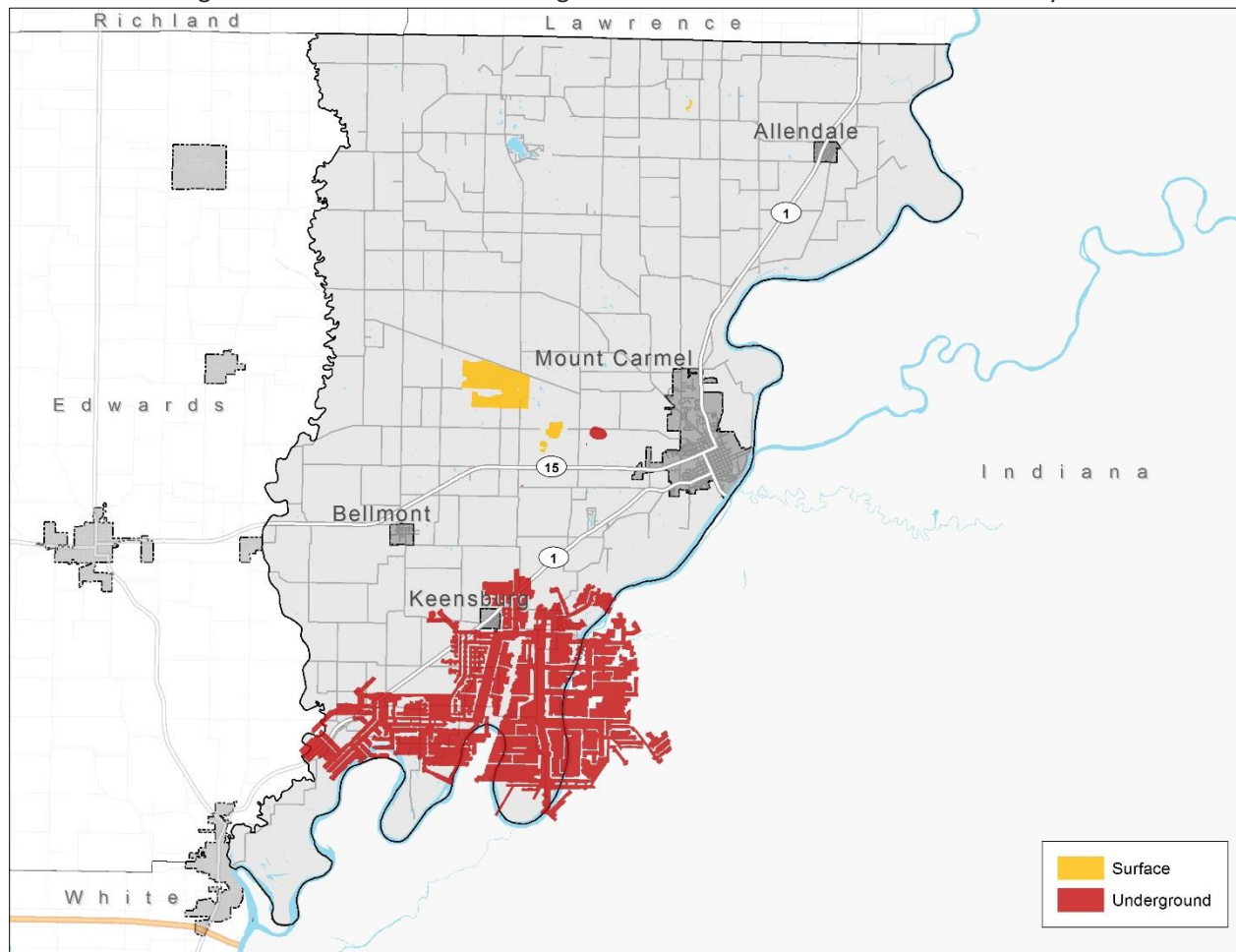
Figure 4-25. Distribution of Underground and Surface Mines in Wabash County
