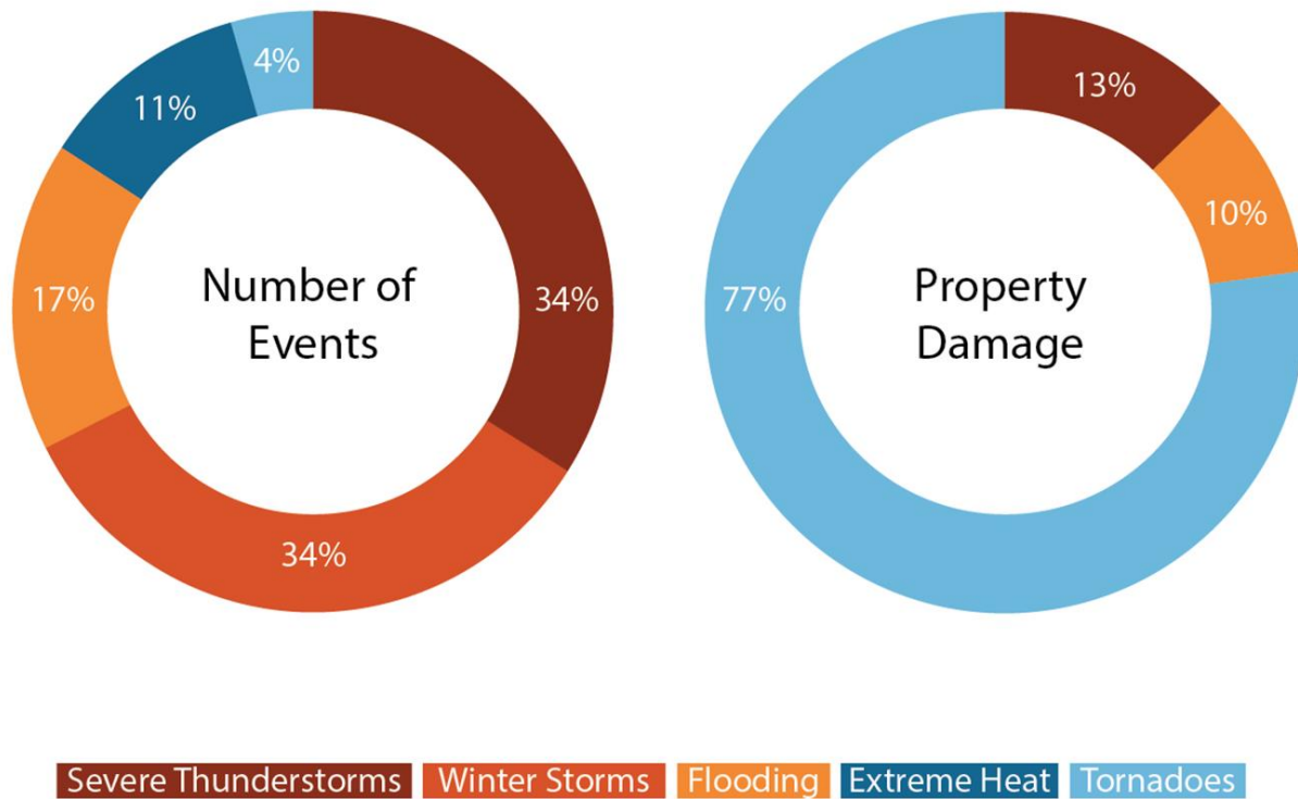
Figure 4-1. Distribution of NCDC Meteorological Hazards for Wabash County
