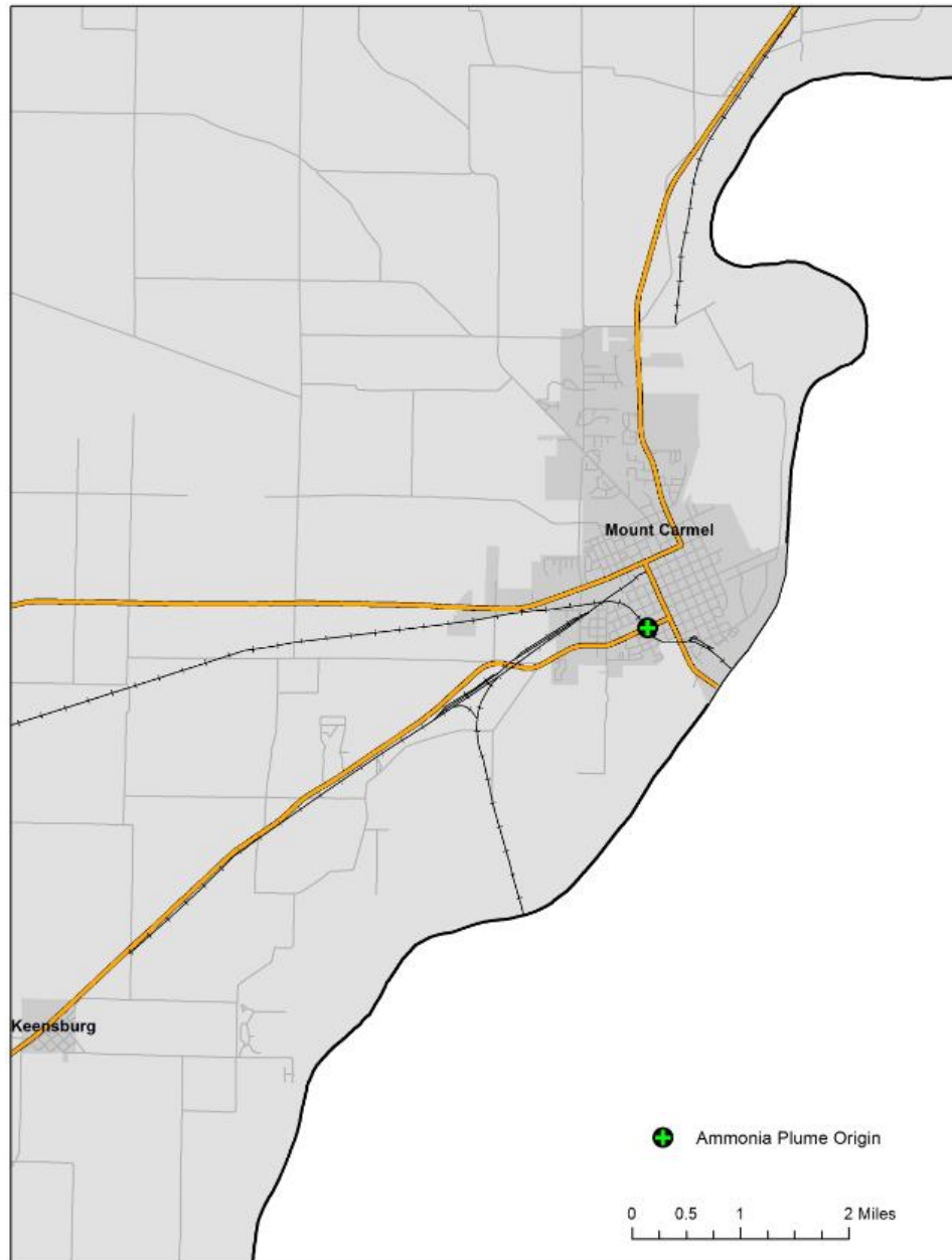
Figure 4-13. ALOHA Modeled Hazardous Chemical Plume Origins in Wabash County
