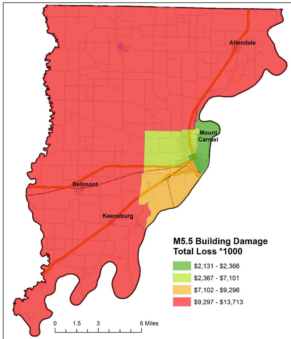
Figure 4-10. Wabash County M5.5 Earthquake Building Economic Losses
