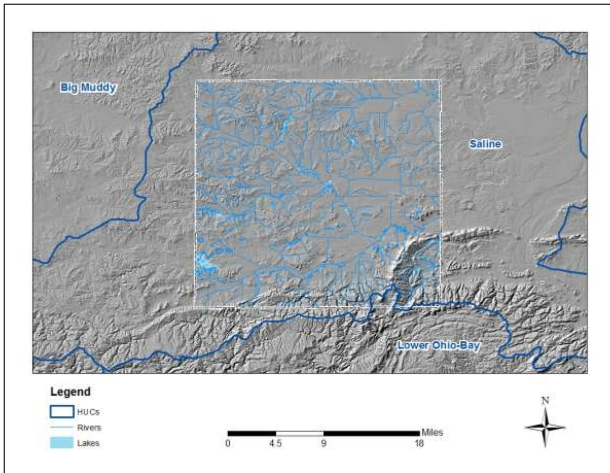
Figure 3-5: Major Lakes and Rivers in Saline County
