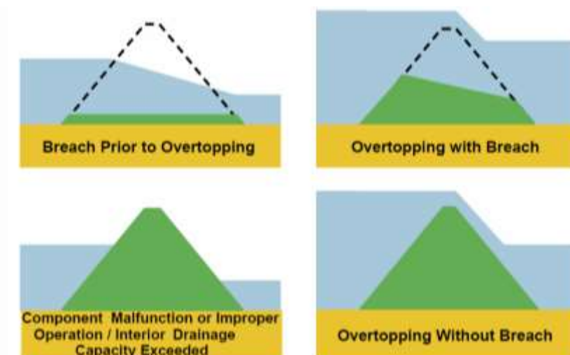
Figure 3-4 Levee Breach Diagram
