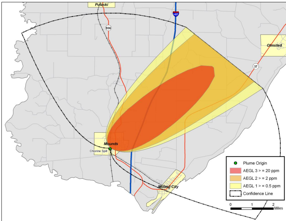
Figure 4-17: ALOHA Plume Footprint Overlaid in ArcGIS
