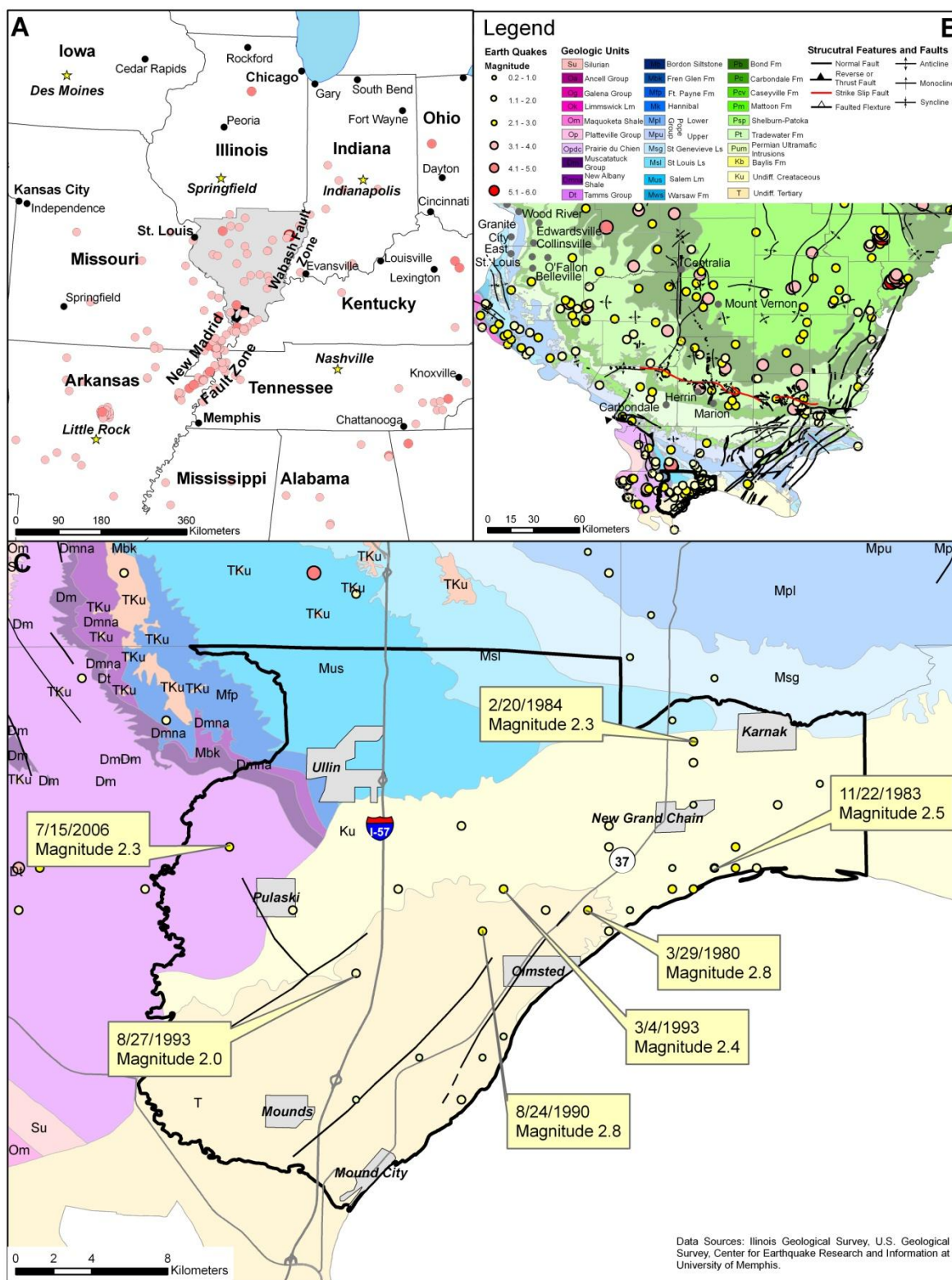
Figure 4-10 a, b, c: Pulaski County Earthquakes
