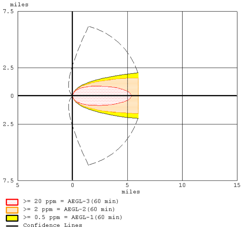
Figure 4-16: Plume Footprint Generated by ALOHA
