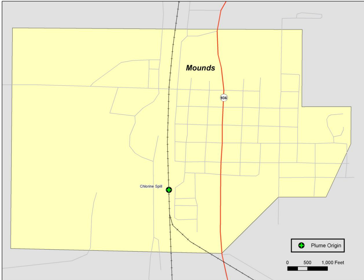
Figure 4-14: Location of Chemical Release
