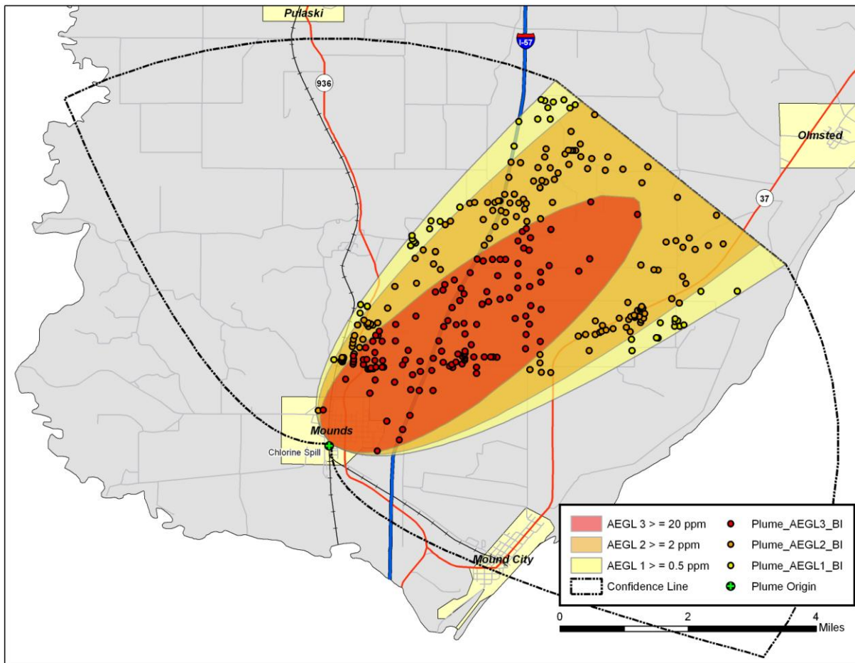
Figure 4-18: Pulaski County Building Inventory Classified By Plume Footprint
