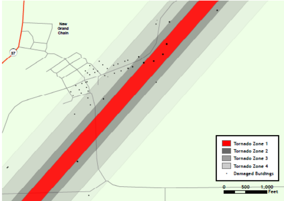
Figure 4-3: Modeled EF4 Tornado Damage Buffers in Pulaski County
