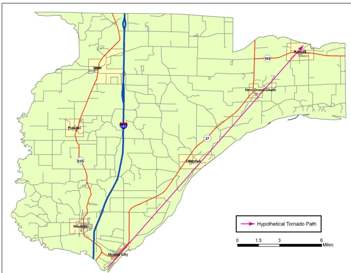
Figure 4-2: Hypothetical EF4 Tornado Path in Pulaski County
