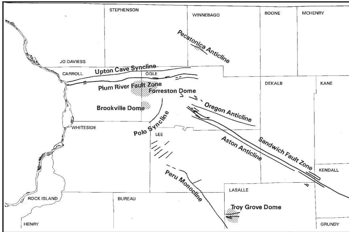
Figure 57 Geological Structures in Northern Illinois
