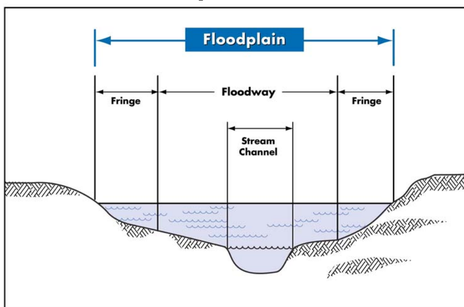
Figure 21 Floodplain Illustration
