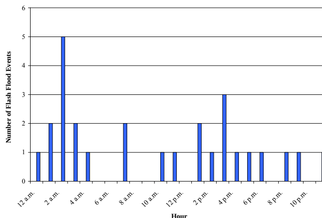
Figure 25 Ogle County Flash Flood Events by Hour – 1979 through 2009
