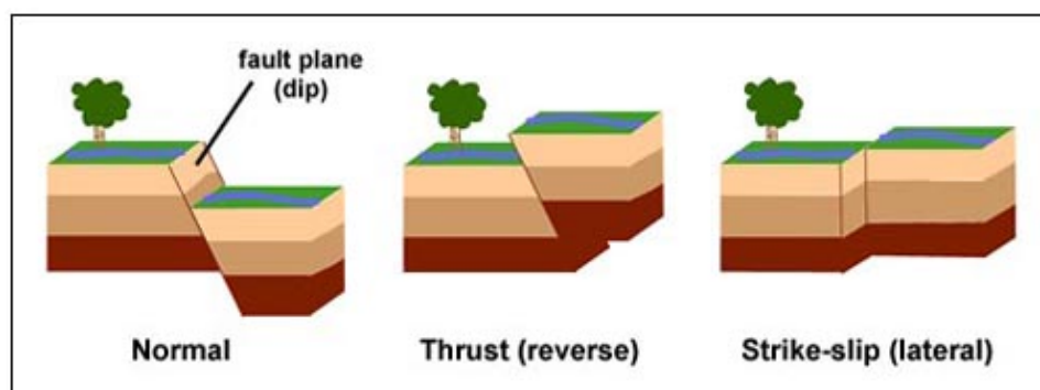
Figure 53 Fault Illustration
