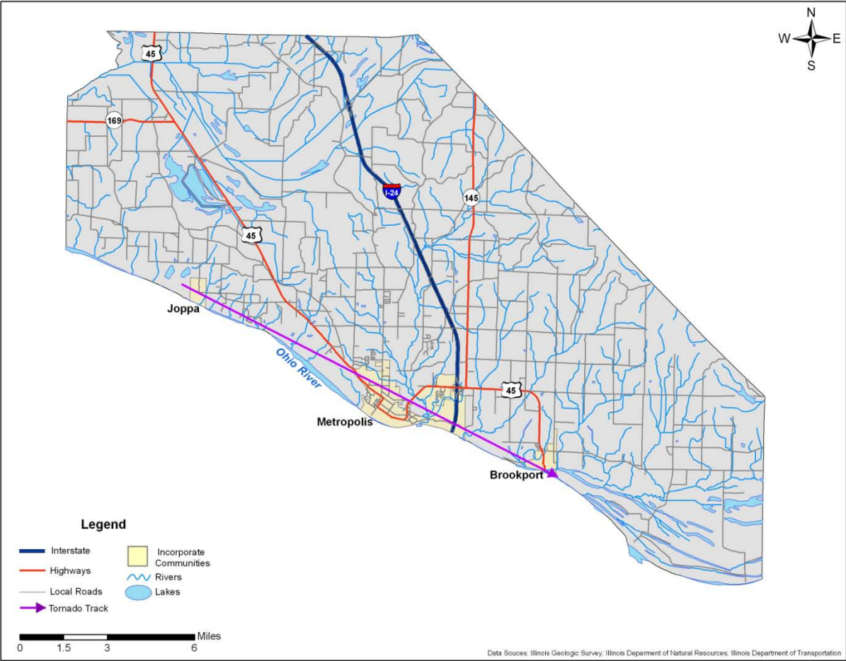
Figure 4-2: Hypothetical F-4 Tornado Path in Massac County
