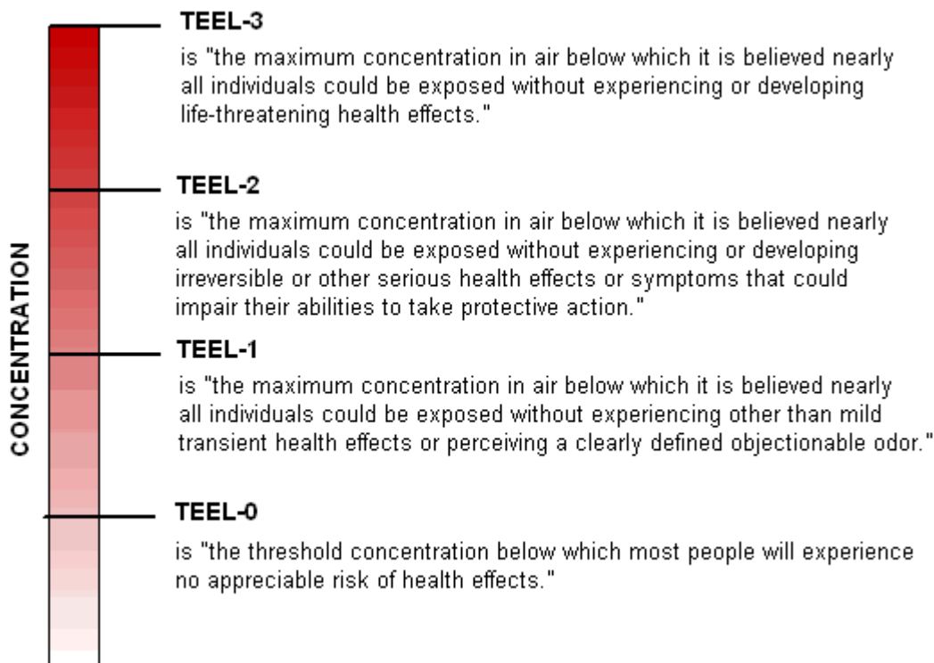
Figure 4-19: TEEL Concentration Tiers
