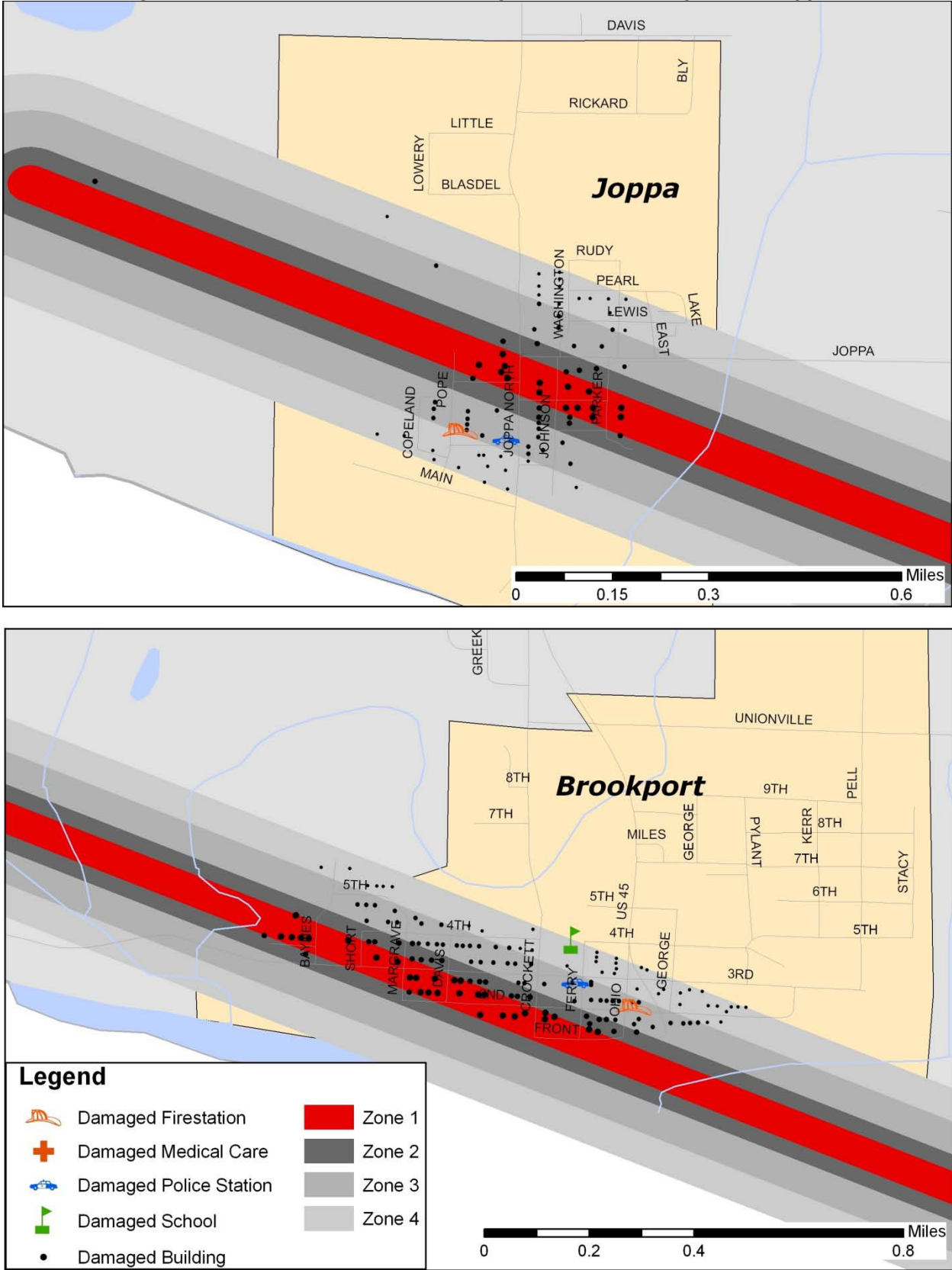
Figure 4-4: Modeled F-4 Tornado Damage Buffers in Brookport and Joppa
