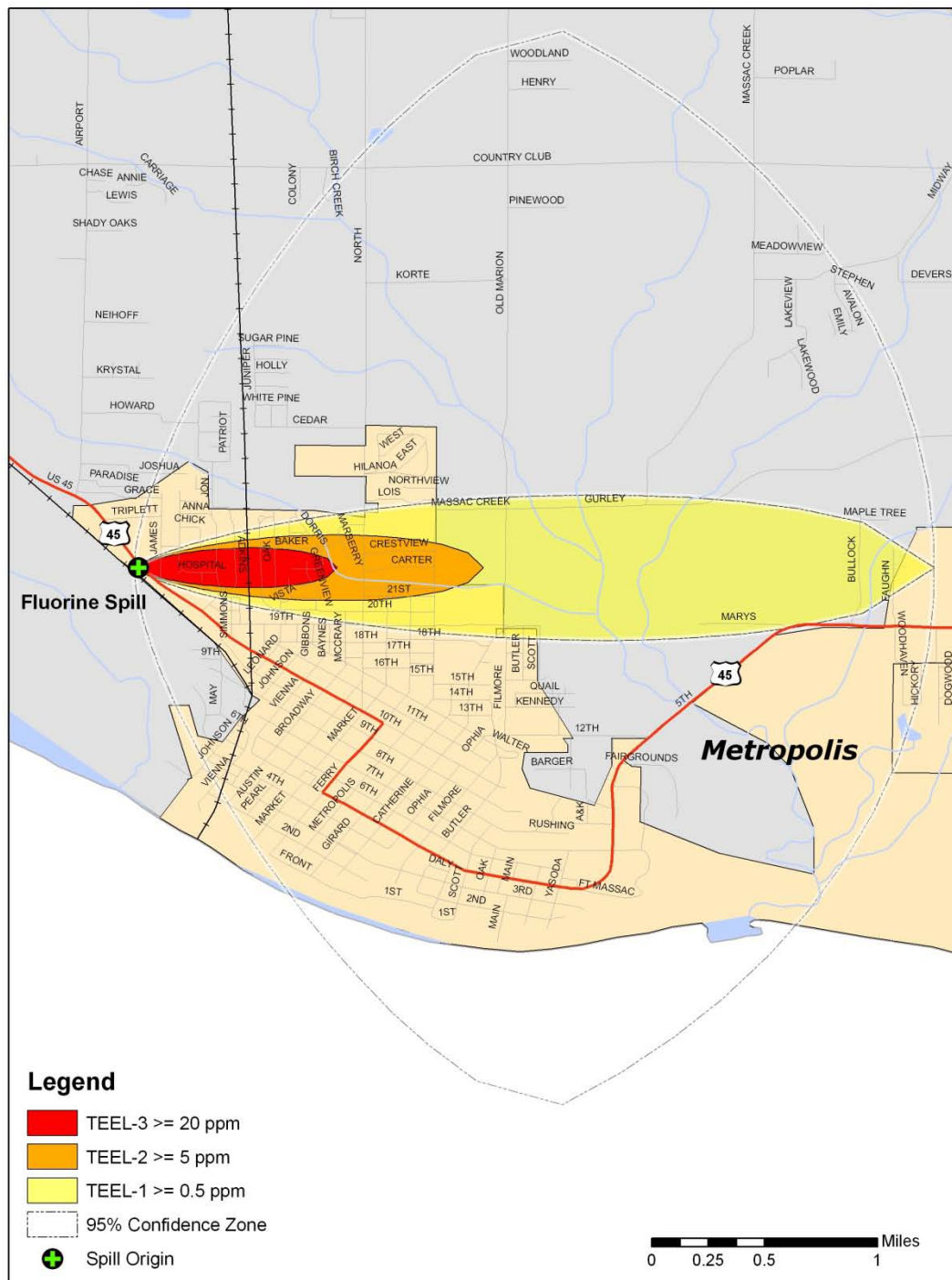
Figure 4-20: ALOHA Plume Footprint Overlaid in ArcGIS
