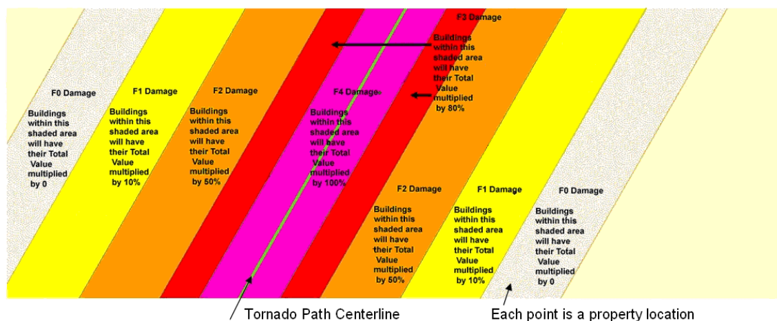
Figure 4-1: GIS Analysis Using Tornado Buffers
