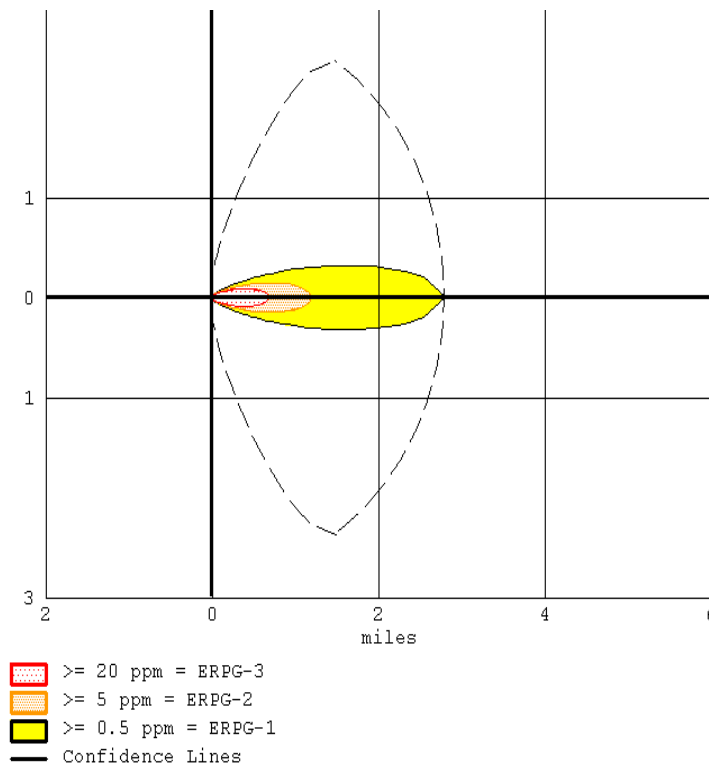
Figure 4-18: Plume Footprint Generated by ALOHA
