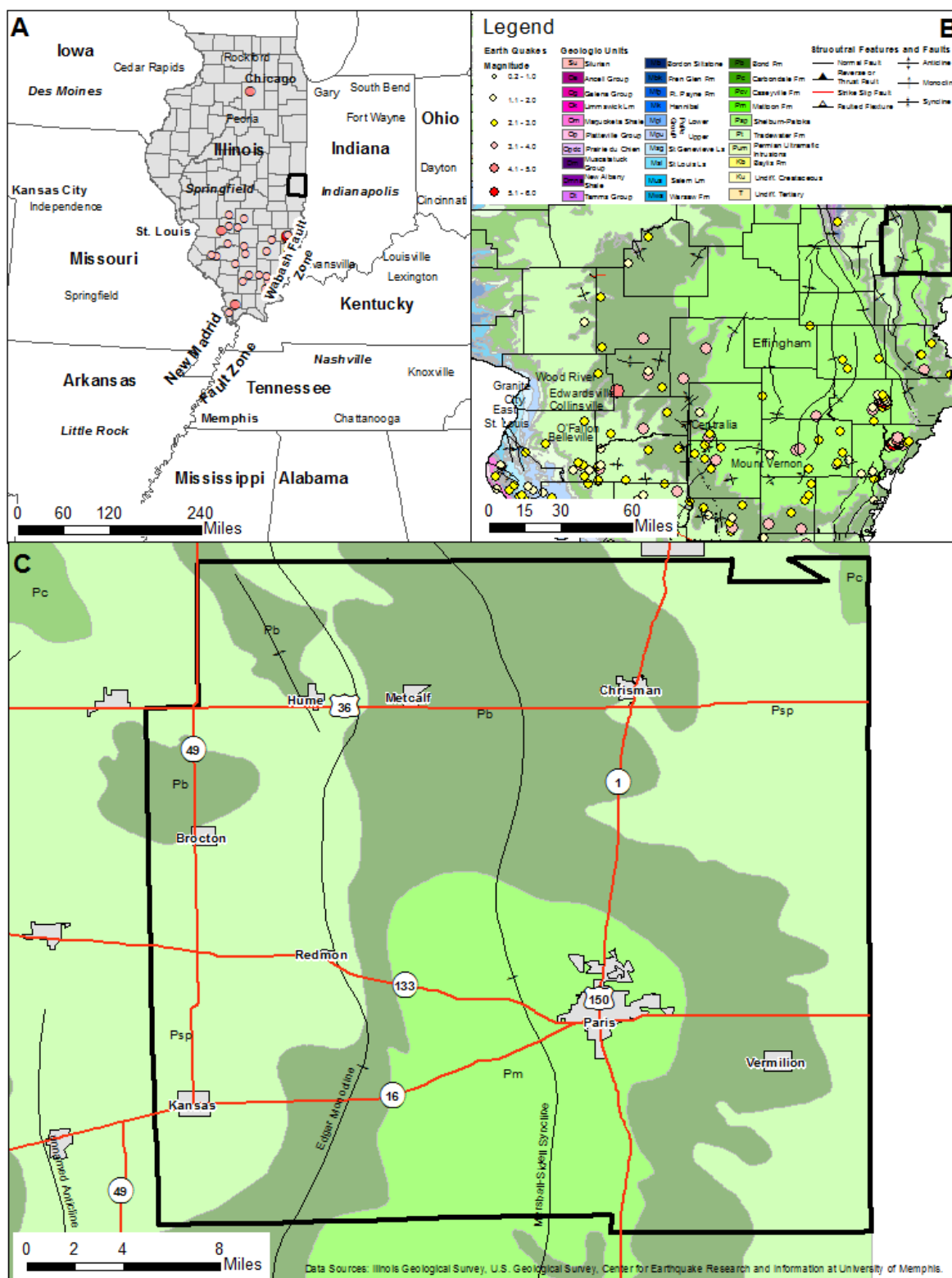
Figure 4-29: Recorded Earthquakes in the U.S. Midwest and Geology of Edgar County
