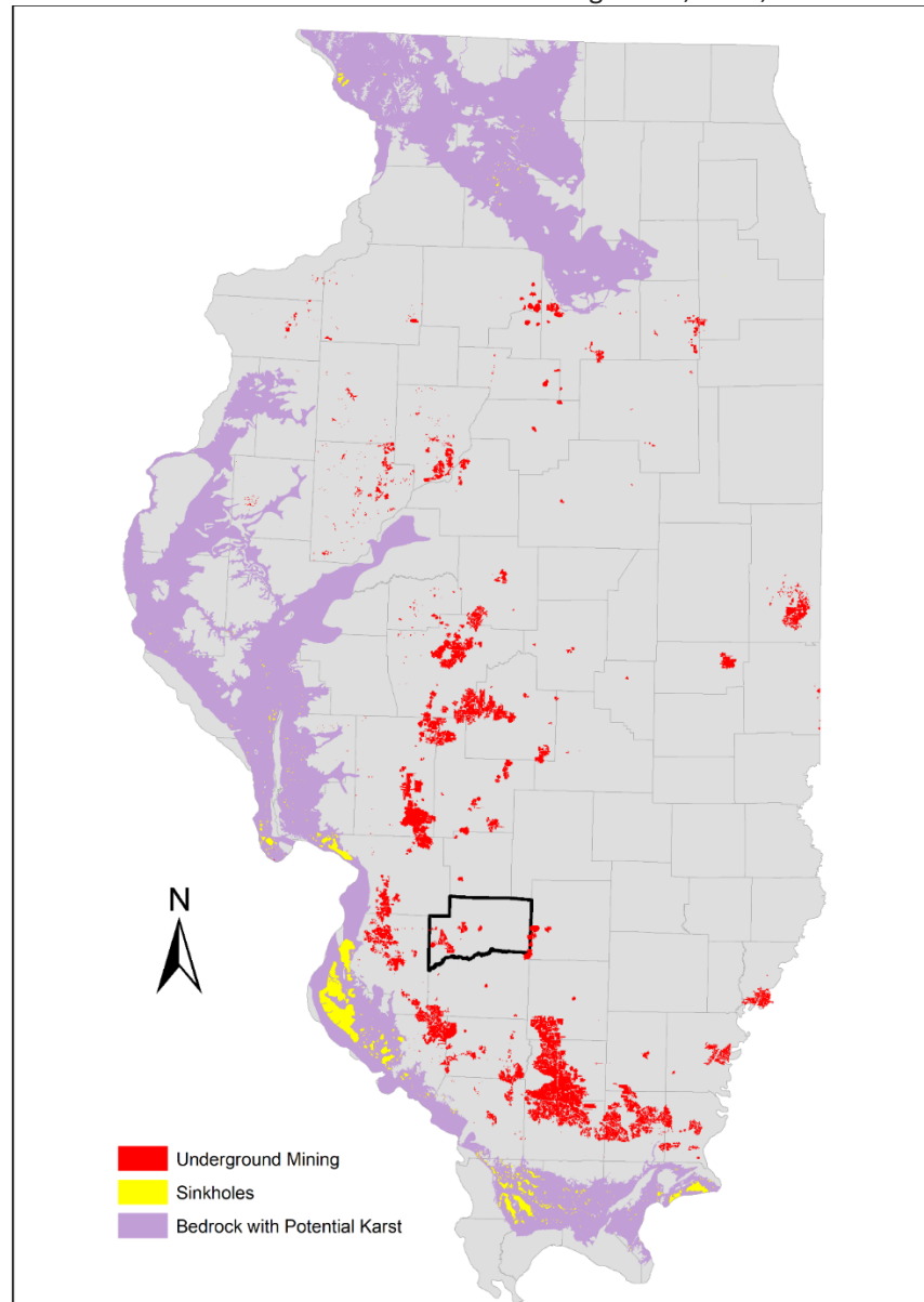
Figure 4-13. Distribution of Bedrock with Potential Coal Bearing Strata, Karst, Sinkholes and Mining Efforts
