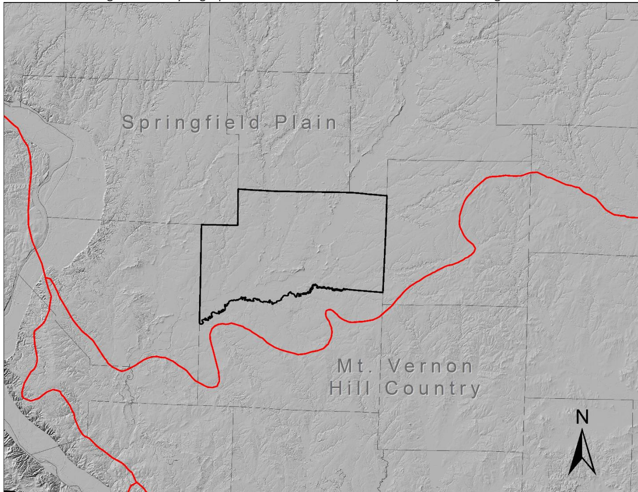
Figure 3-4. Physiographic Divisions of Clinton County and Surrounding Terrain
