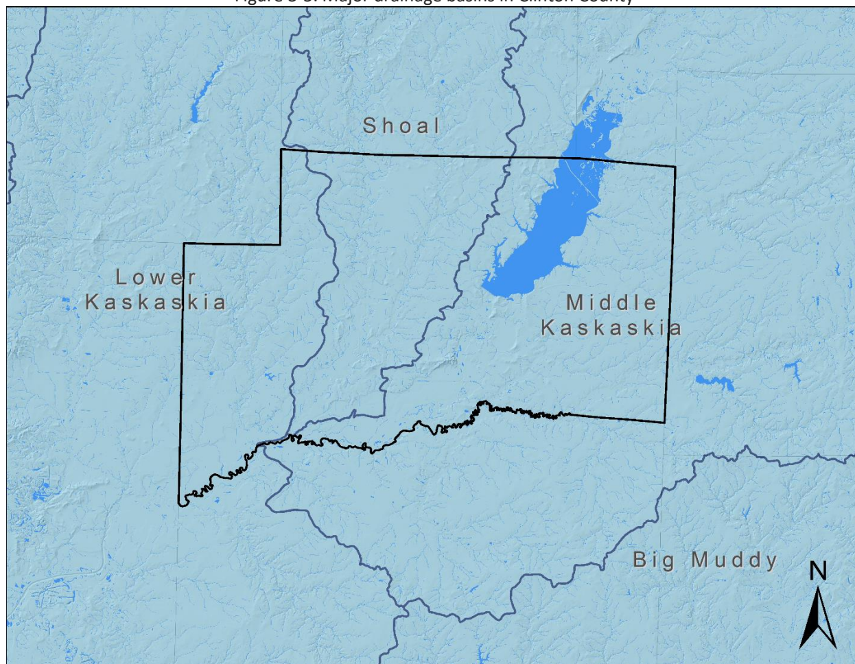
Figure 3-5. Major drainage basins in Clinton County
