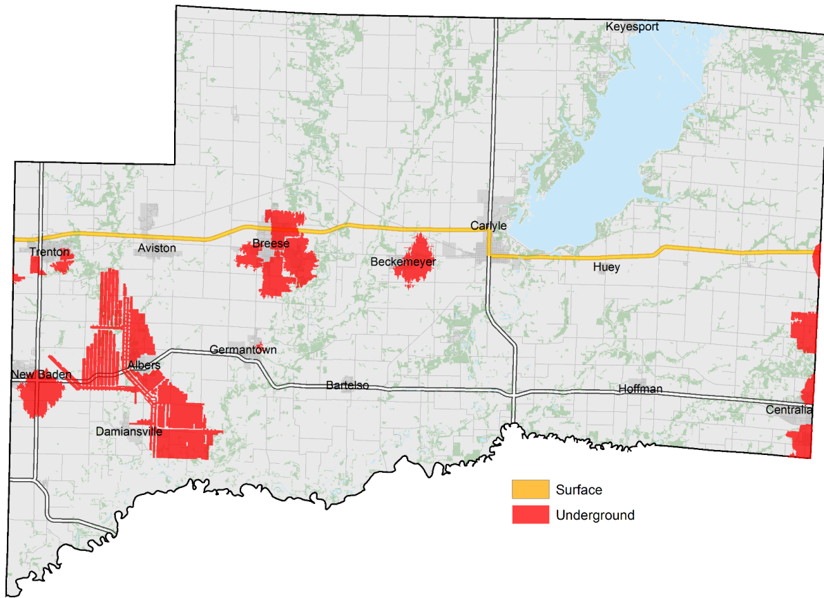
Figure 4-14. Distribution of potential karst bedrock, sinkholes, and underground mines in Clinton County
