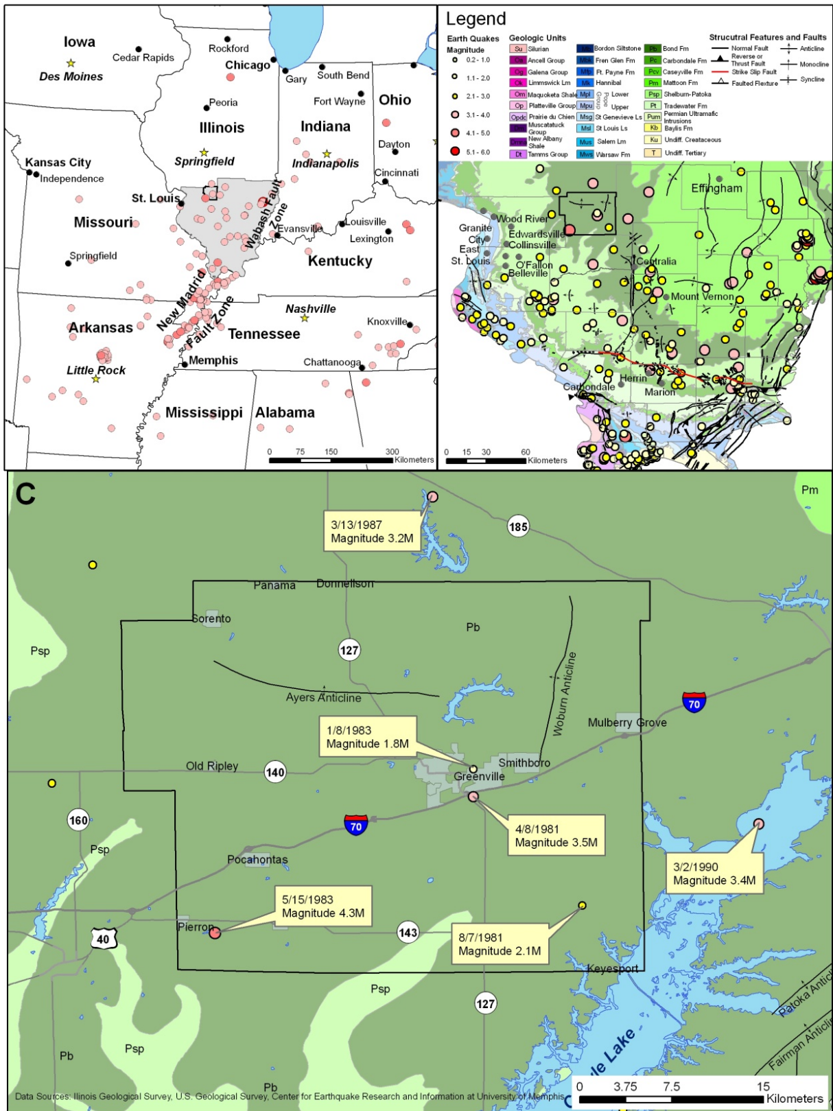
Figure 4-6 a, b, c: Bond County Earthquakes
