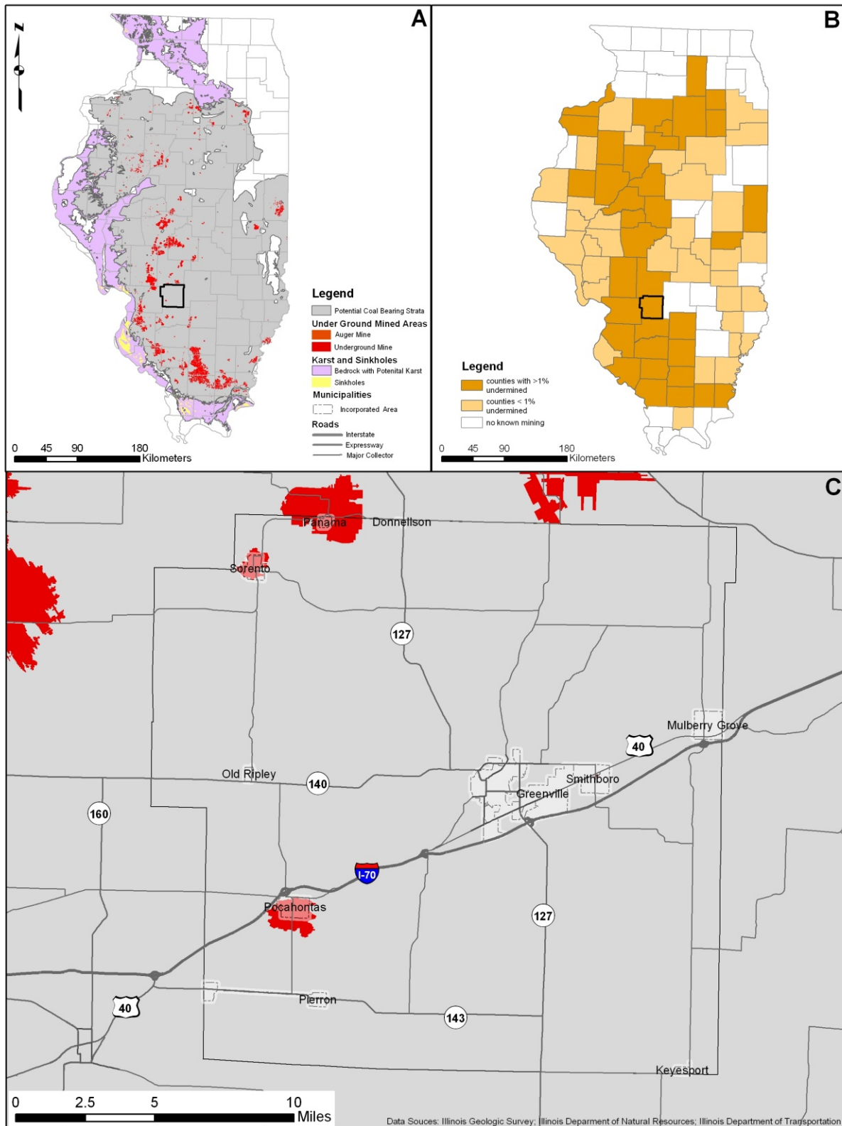
Figures 4-16a, 4-16b, and 4-16c: Maps of Statewide and Countywide Areas with Subsidence Hazard Potential
