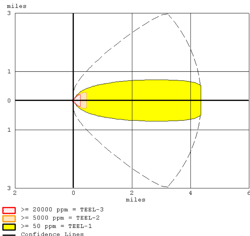
Figure 4-21: Plume Footprint Generated by ALOHA
